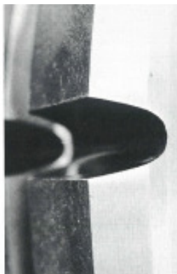
Back gouging on a longitudinal weld seam.
